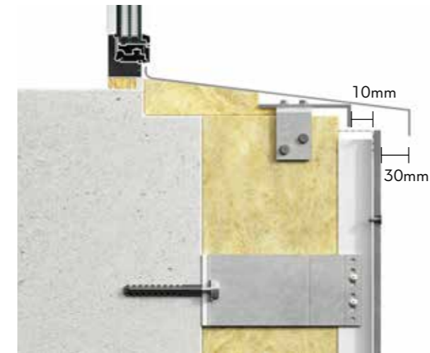
Vertical view: Window Sill
