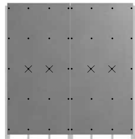
Example: Vertically mounted boards with two intermediate profile
