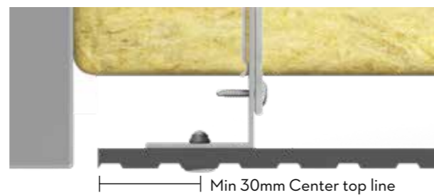
Fig. 4. Cembrit Patina Inline installation on cut to size board.
