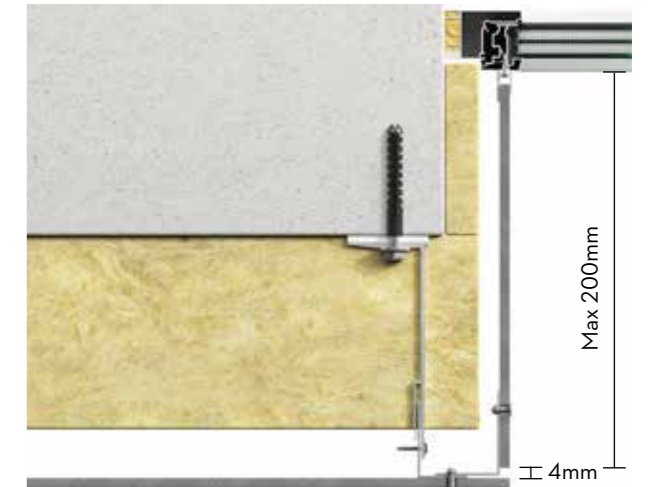
Horizontal view: Window jambs
