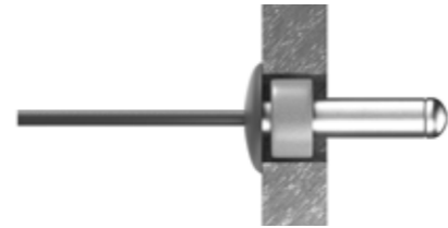
X : Fixing position hole diameter Ø10 mm (Aluminium). X : Fixing position hole diameter Ø9 mm (Steel). Insert a Cembrit Fixing Sleeve in the hole before the rivet is fixed.
